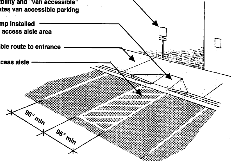
Diagram of Van Accessible Parking Space Elements
