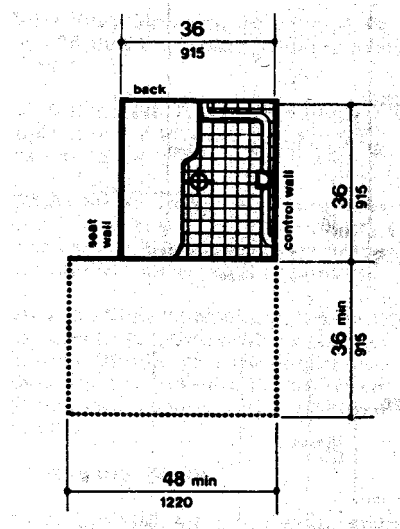
ADA Stds. Figure 35(a) - Small Shower Size and Clearances
