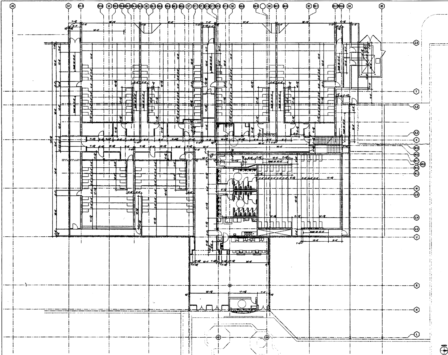
01 FIRST FLOOR DIMENSION CONTROL PLAN
