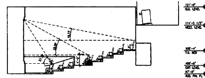
04 AUDITORIUM 1 VIEWING ANGLE - REFERENCE ONLY
