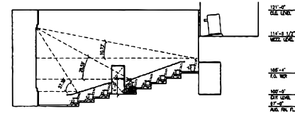
02 AUDITORIUM 2 VIEWING ANGLE - REFERENCE ONLY
