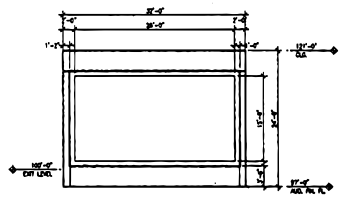
19 AUDITORIUM 1 ELEVATION
