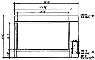
20 AUD 1 SCREEN ELEVATION
