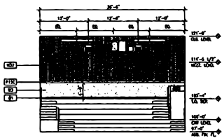
19 AUDITORIUM 1 ELEVATION
