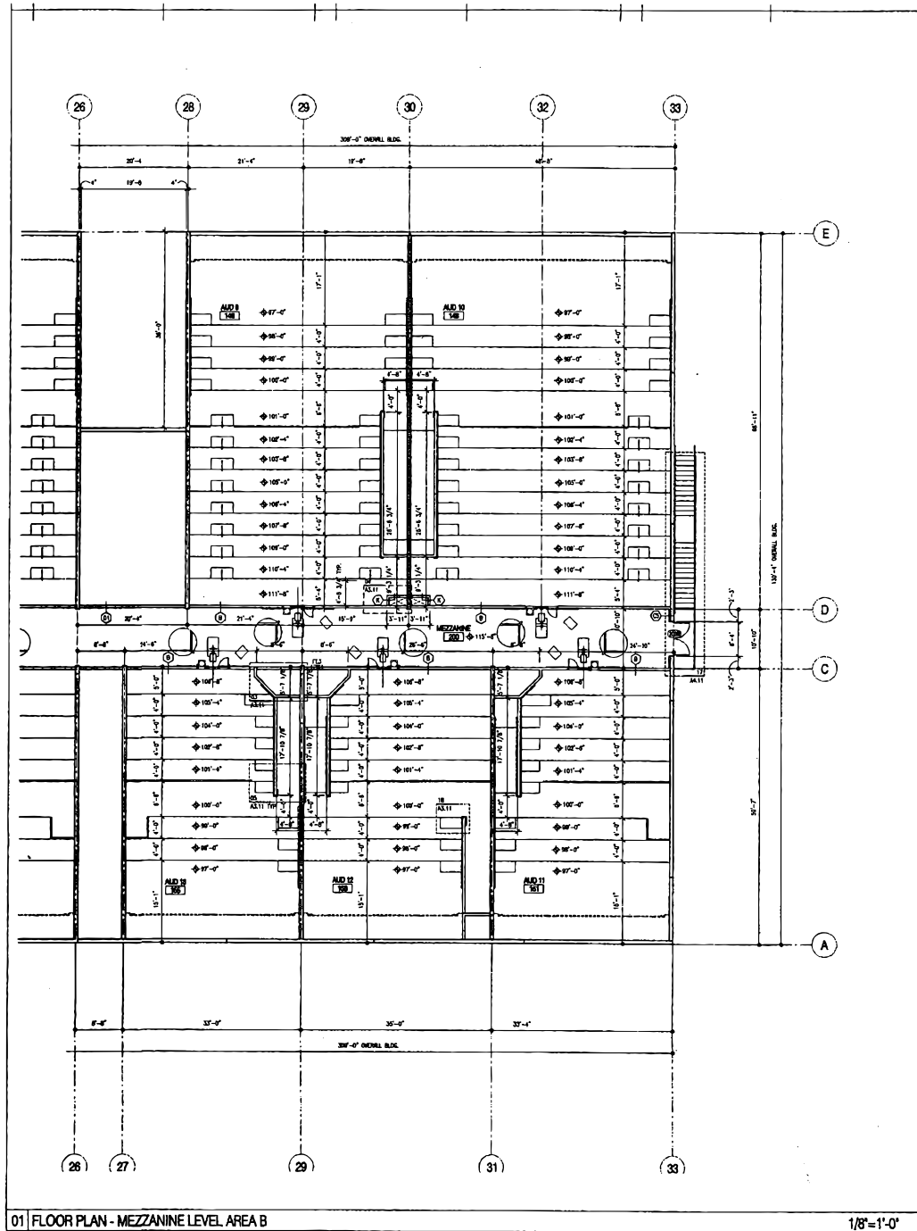
01 FLOOR PLAN - MEZZANINE LEVEL, AREA B
