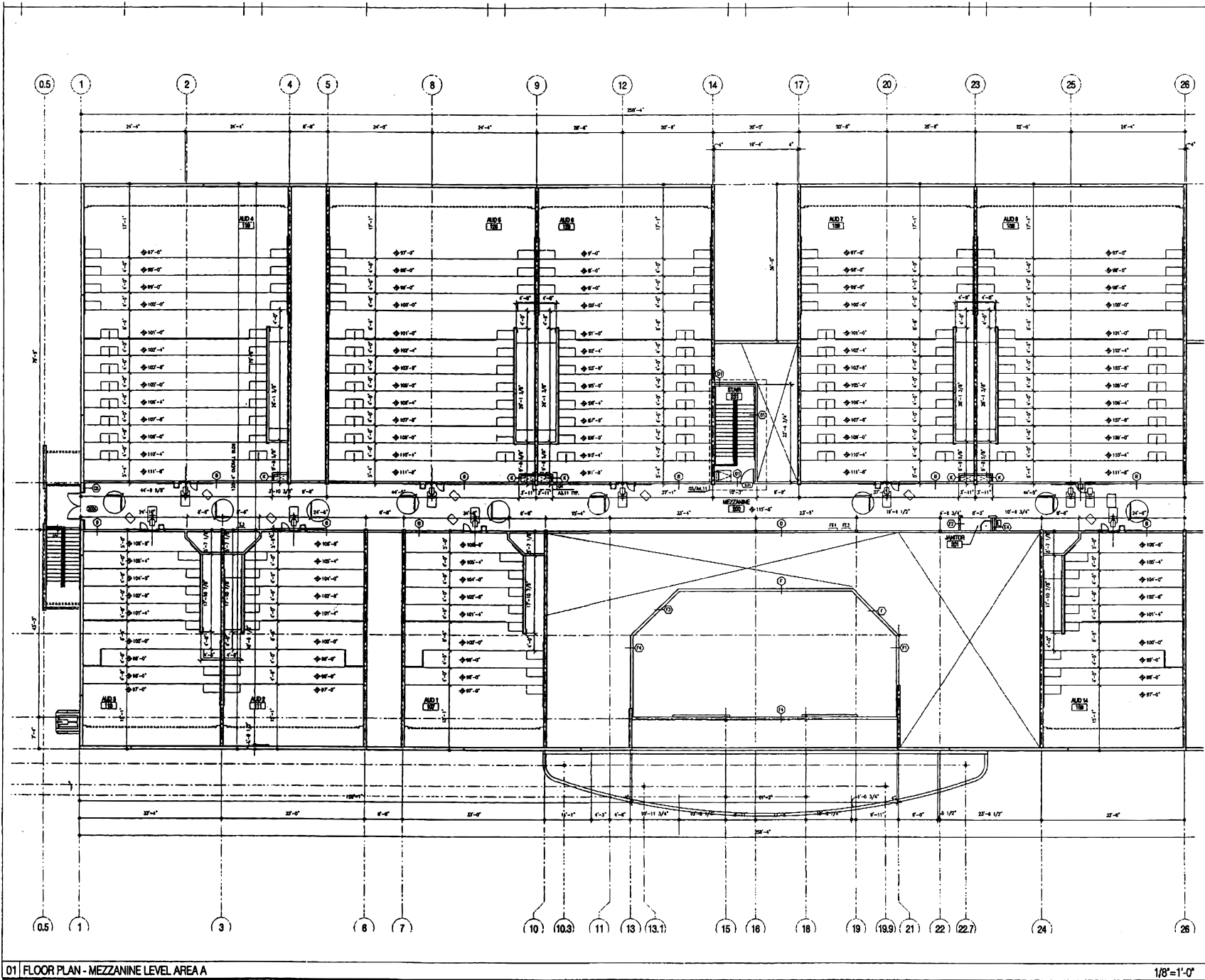
01 FLOOR PLAN - MEZZANINE LEVEL AREA A
