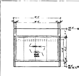
20 AUD. 14 SCREEN ELEVATION 1/8"=1'-0"
