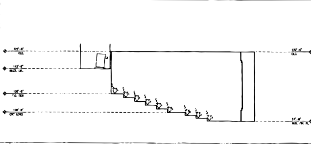
09 AUDITORIUM 2 INTERIOR ELEVATION 1/8"=1'-0"
