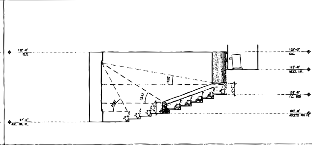
01 AUDITORIUM 2 INTERIOR ELEVATION 1/8"=1'-0"
