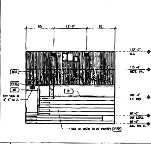
19 AUD. 14 INTERIOR ELEVATION 1/8"=1'-0"
